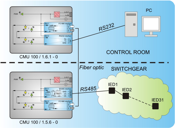
Picture 2: CMU 100 / x.6.1 - 0 typical application
