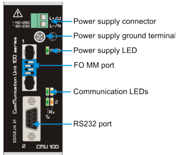
Picture 3: CMU 100 / x.6.1 - 0 front view
