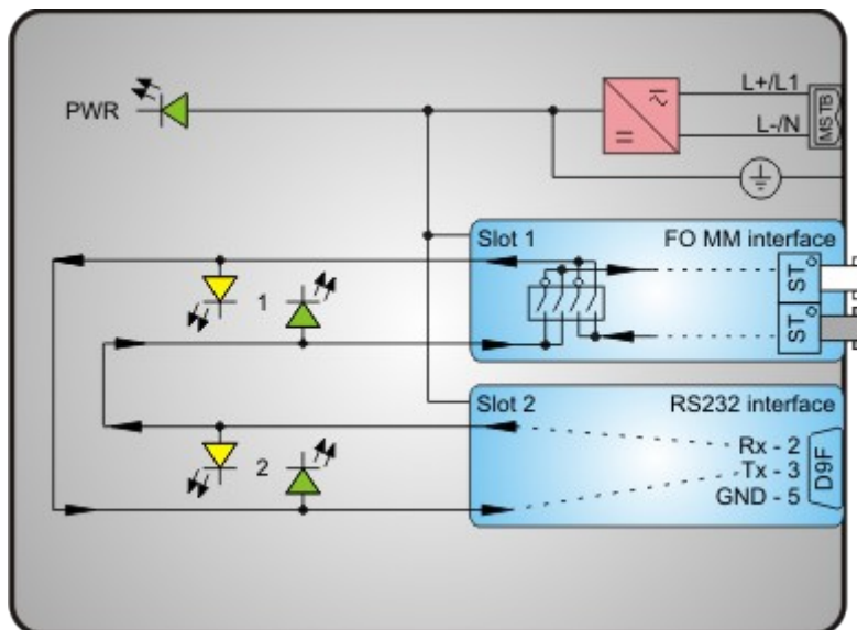
Picture 6: CMU 100 / x.6.1 - 0 schematic
