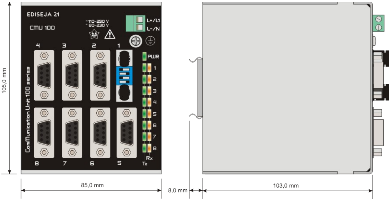
Picture 8: Dimensions
