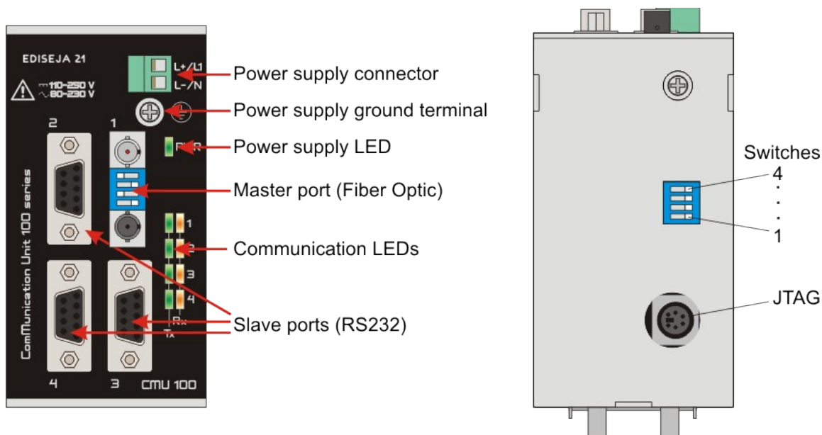
Picture 4: Front view (left) & bottom view (right)
