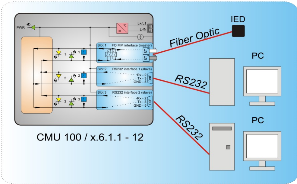
Picture 2: CMU 100 / x.6.1.1 - 12 typical application
