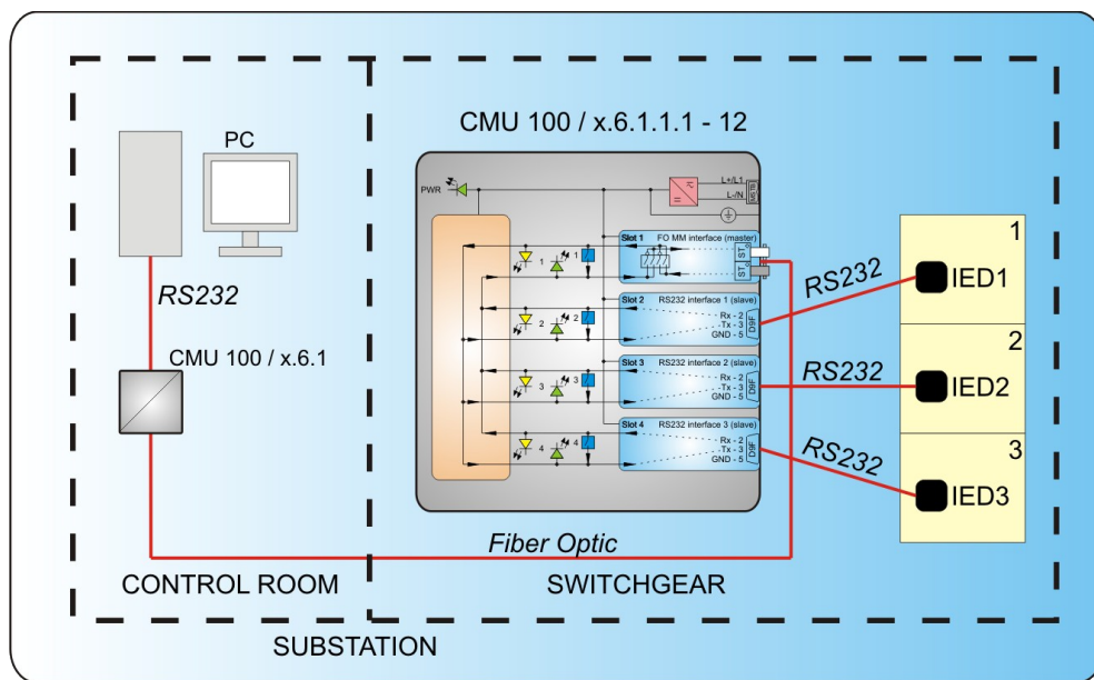
Picture 3: CMU 100 / x.6.1.1.1 - 12 typical application
