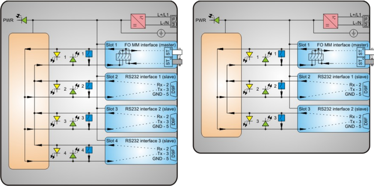
Picture 7: CMU 100 / x.6.1.1.1 - 12 (left) and CMU 100 / x.6.1.1 - 12 (right) schematic
