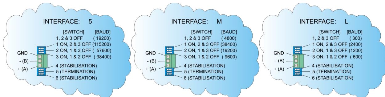
Picture 5: RS485 interface board appearance with switch settings
