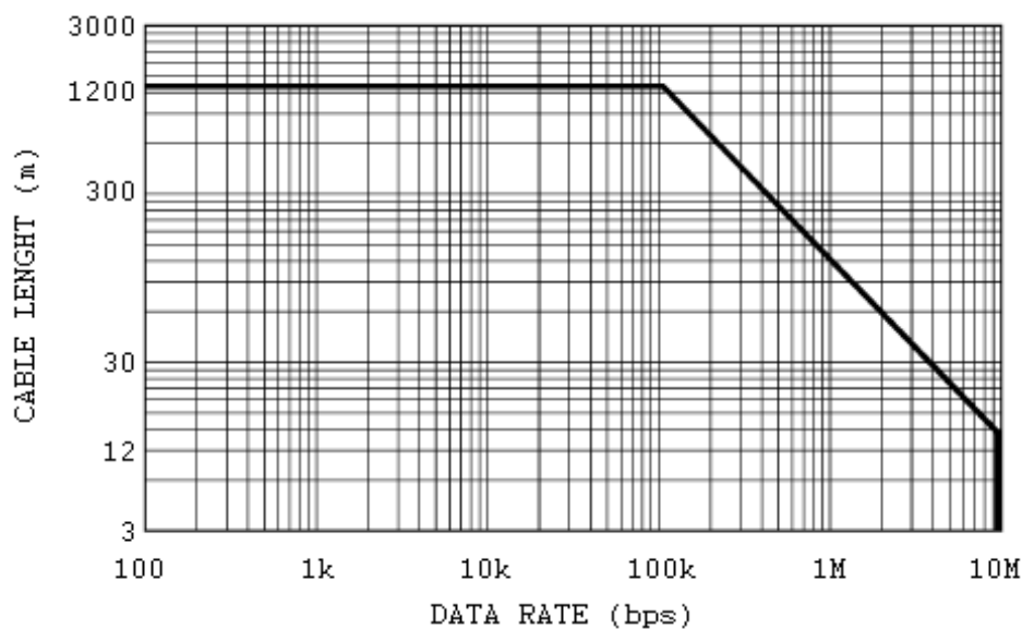
Picture 6: Standard data rate vs cable lenght
