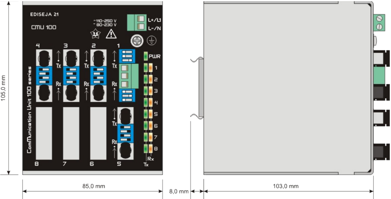
Picture 11: CMU 100 / 2.5.6.6.6.6-12 dimensions
