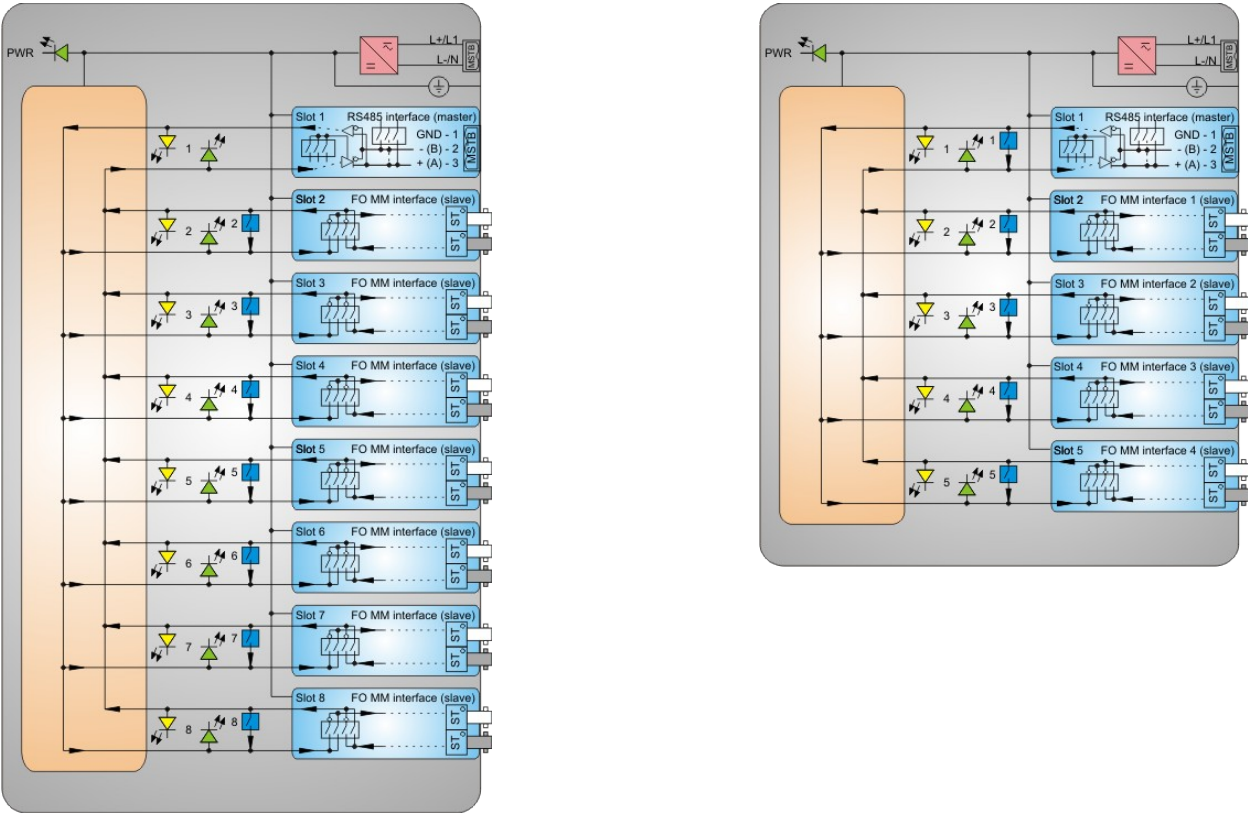
Picture 8: CMU 100 / 2.5.6.6.6.6.6.6 – 12 (left) and CMU 100 / 2.5.6.6.6.6 - 12 (right) general diagram
