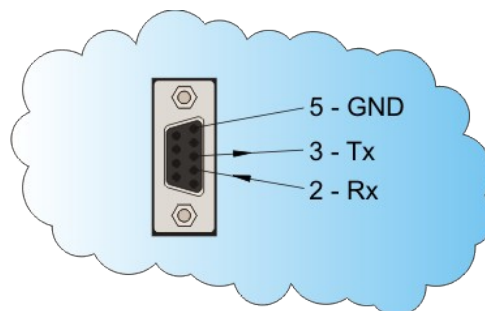
Picture 7: DB9 Female connector
