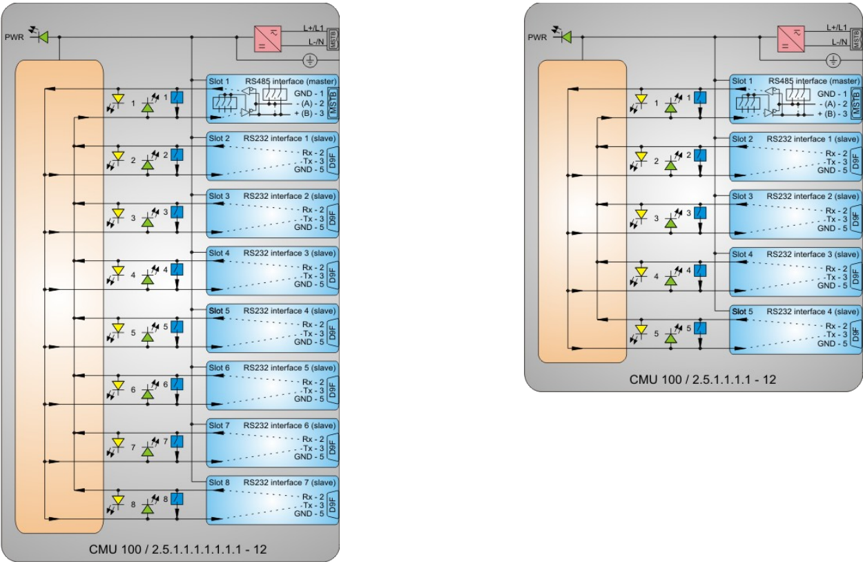
Picture 8: CMU 100 / 2.5.1.1.1.1.1 - 12 (left) and CMU 100 / 2.5.1.1.1.1 - 12 (right) general diagram
