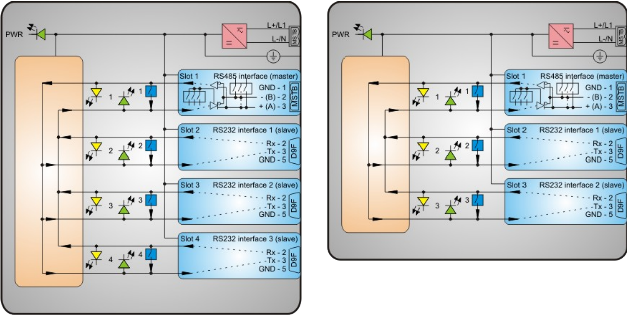
Picture 9: CMU 100 / x.5.1.1.1 - 12 (left) and CMU 100 / x.5.1.1 - 12 (right) schematic
