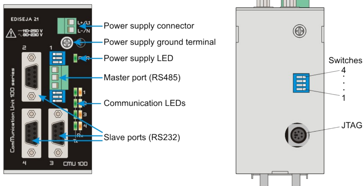
Picture 4: CMU 100 / x.5.1.1.1 - 12 front view (left) & bottom view (right)
