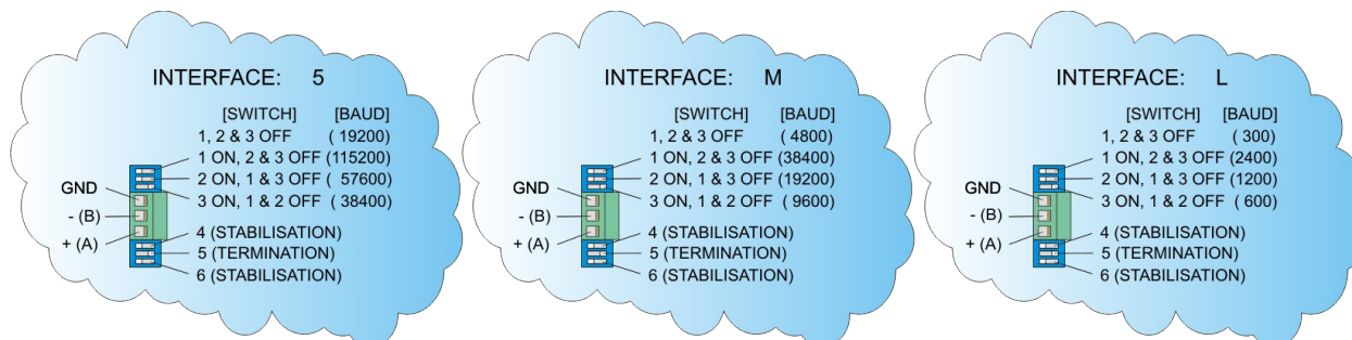
Picture 7: RS485 interface board appearance with switch settings
