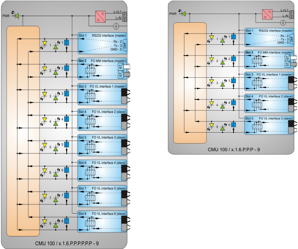
Picture 7: CMU 100 / x.1.6.P.P.P.P.P - 9 schematic (left) & CMU 100 / x.1.6.P.P.P - 9 schematic (right)
