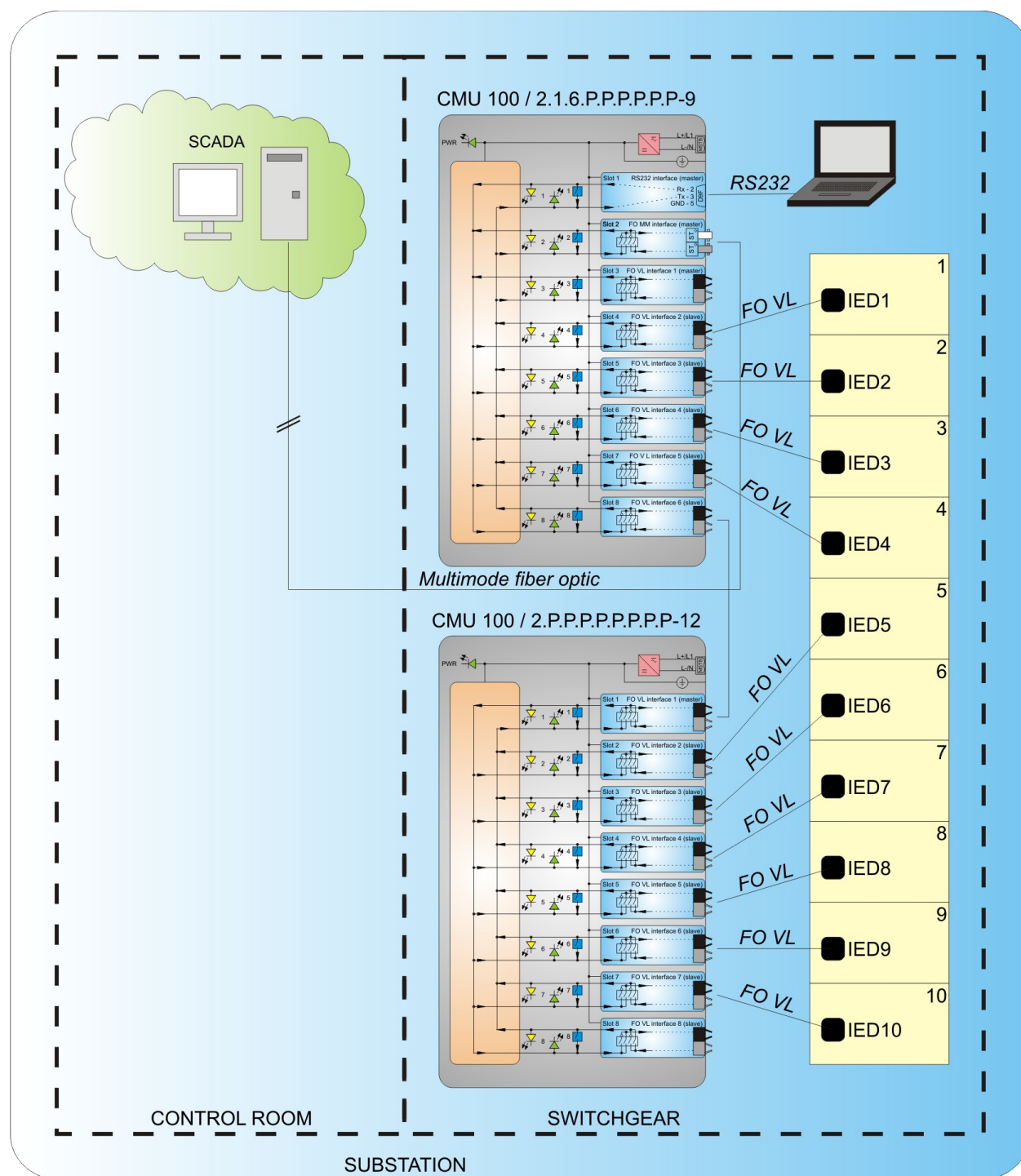
Picture 2: Star coupler typical application
