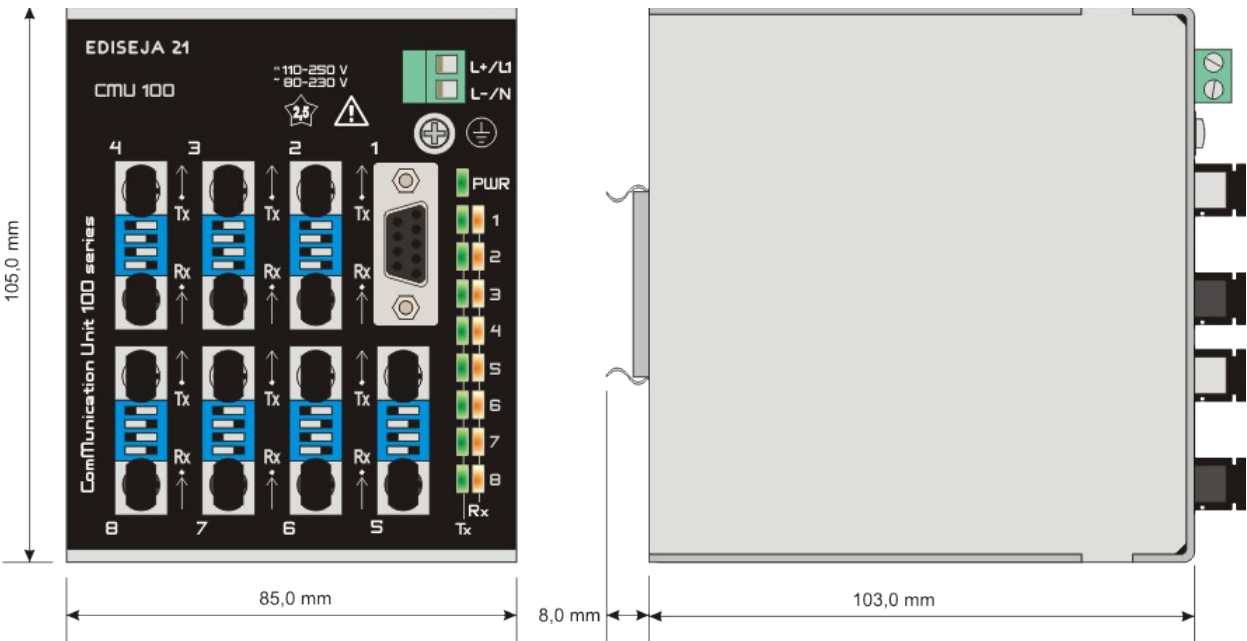
Picture 8: CMU 100 / x.1.6.6.6.6.6.6 - 12 dimensions
