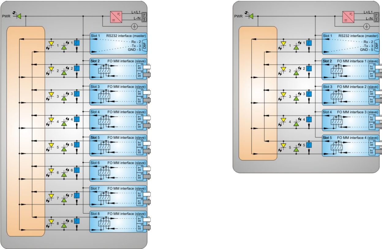
Picture 6: CMU 100 / x.1.6.6.6.6.6.6 - 12 (left) and CMU 100 / x.1.6.6.6.6 - 12 (right) general diagram
