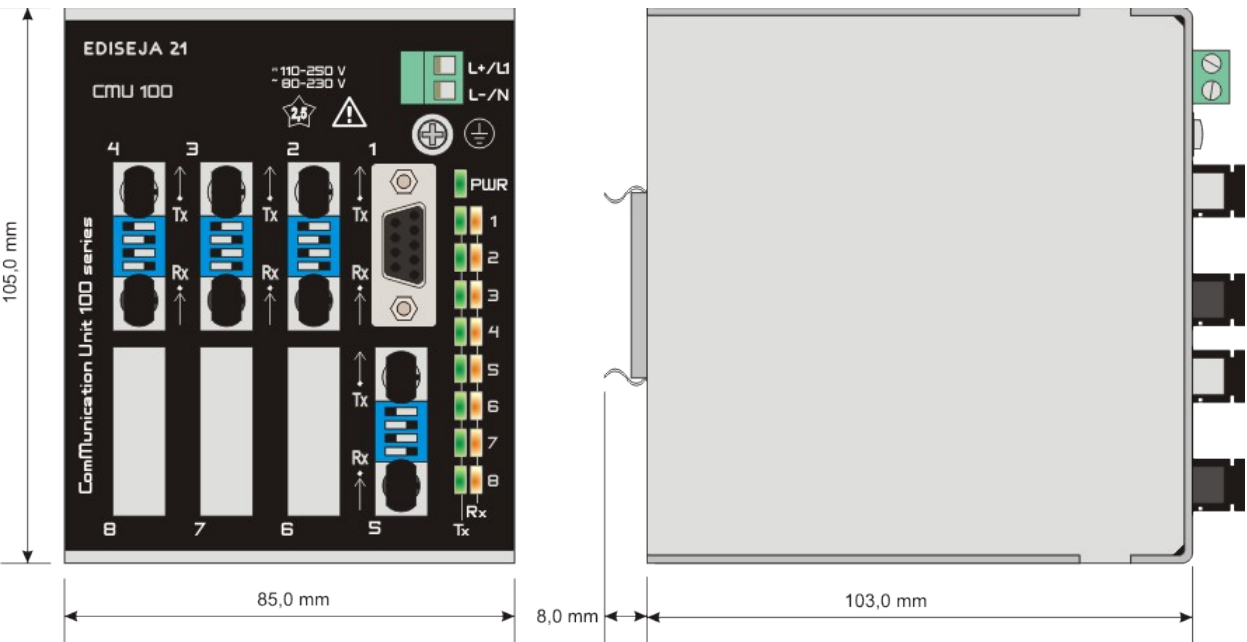
Picture 9: CMU 100 / x.1.6.6.6.6 - 12 dimensions
