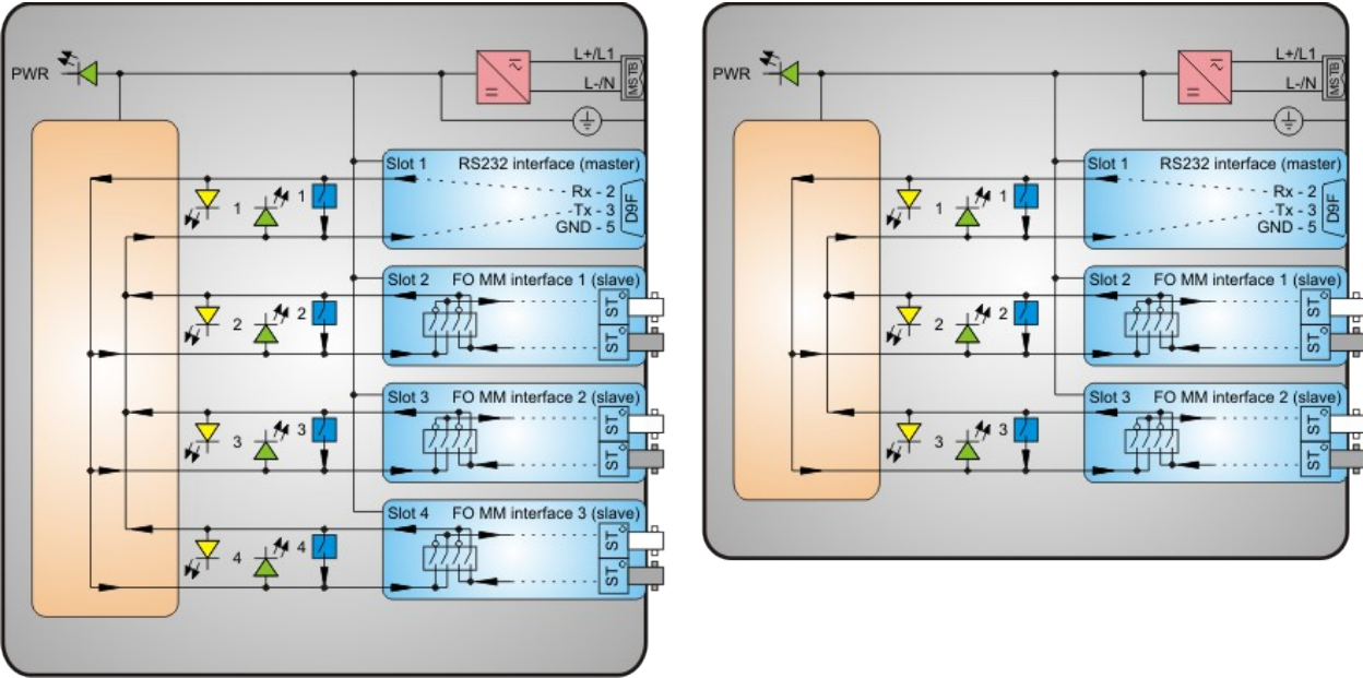
Picture 6: CMU 100 / x.1.6.6.6 - 12 (left) and CMU 100 / x.1.6.6 - 12 (right) schematic
