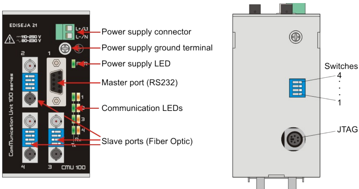
Picture 3: Front view (left) & bottom view (right)
