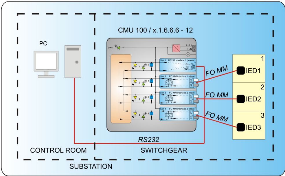
Picture 2: Typical application
