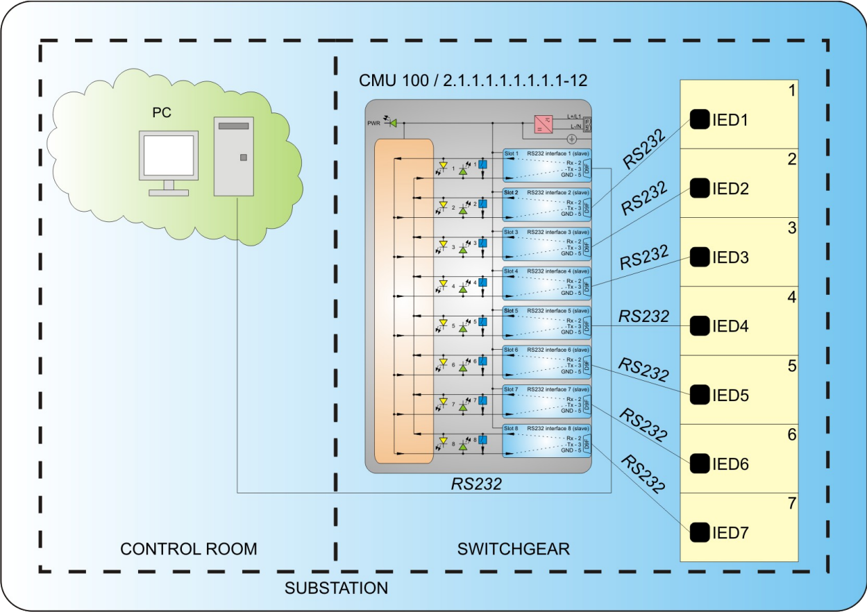
Picture 2: Typical application
