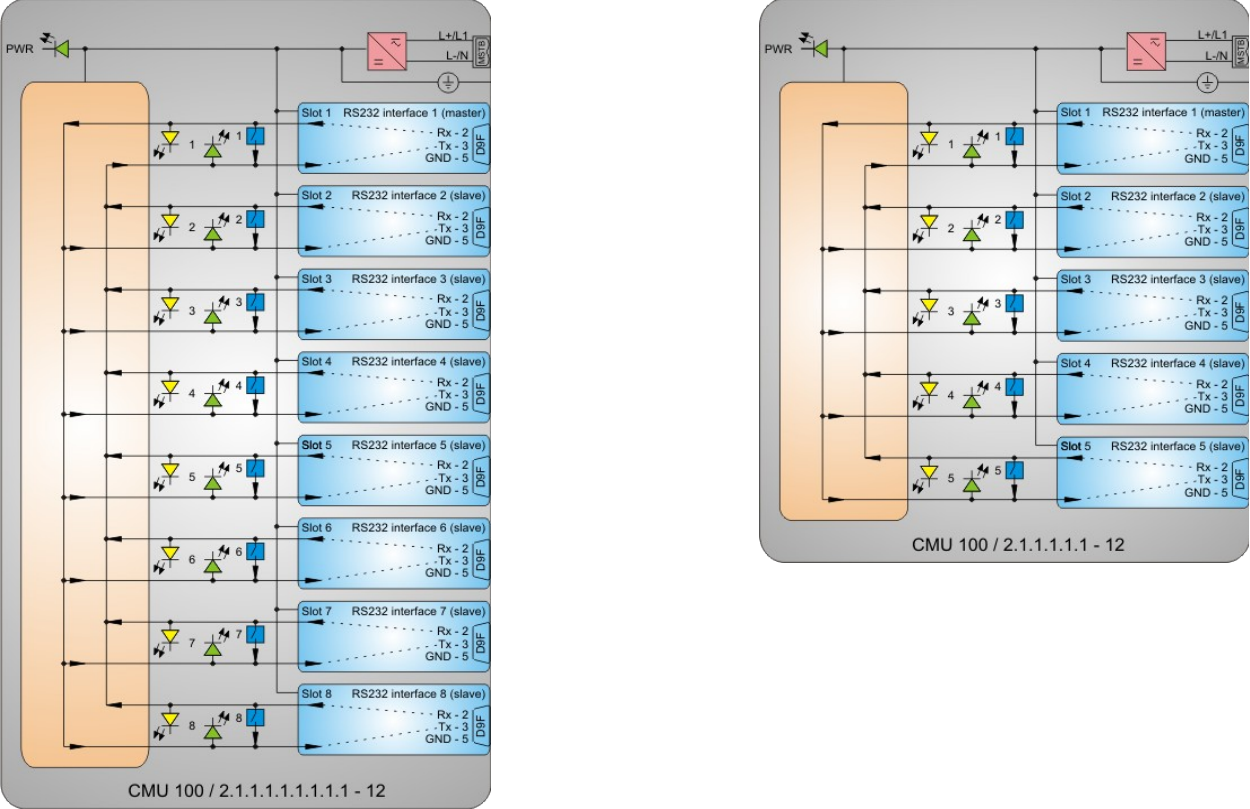
Picture 5: CMU 100 / 2.1.1.1.1.1.1 - 12 (left) and CMU 100 / 2.1.1.1.1.1 - 12 (right) general diagram
