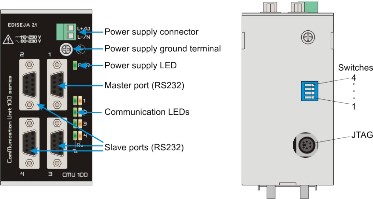
Picture 4: Front view (left) & bottom view (right)
