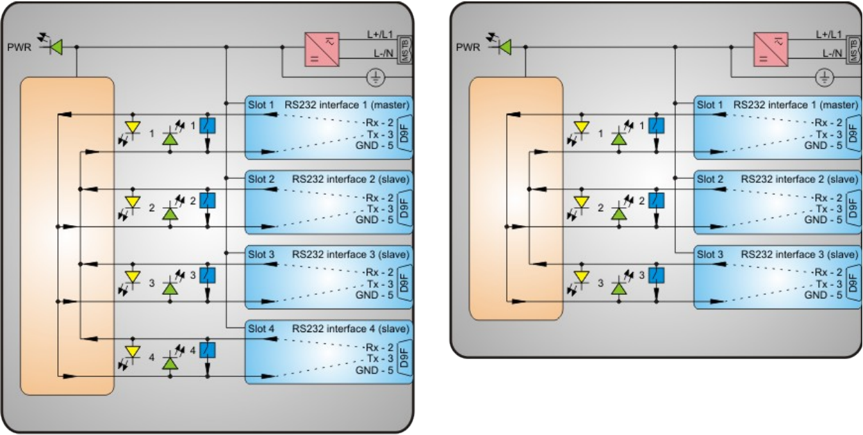
Picture 6: CMU 100 / x.1.1.1.1 - 12 (left) and CMU 100 / x.1.1.1 - 12 (right) schematic
