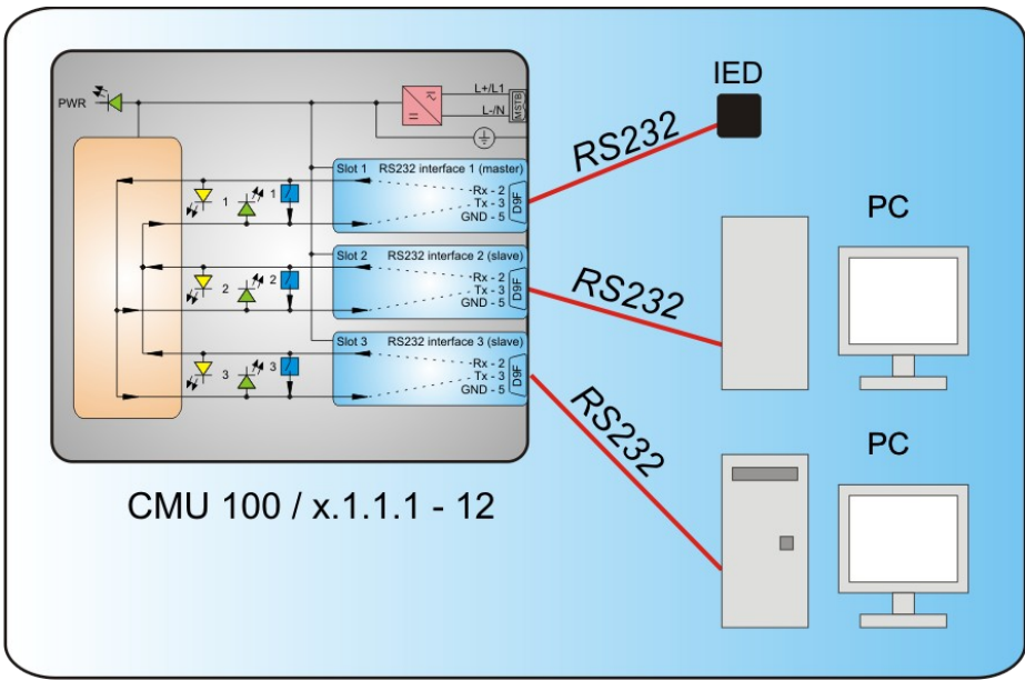
Picture 3: CMU 100 / x.1.1.1 - 12 typical application
