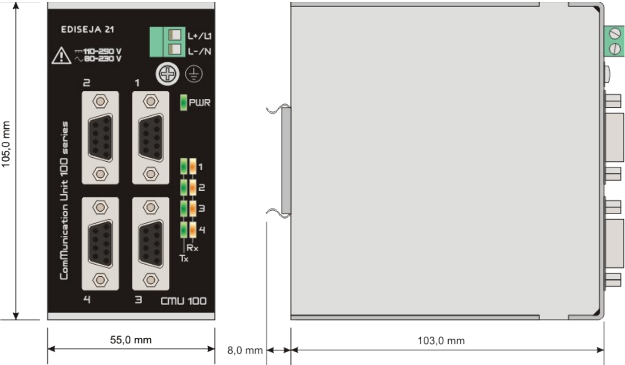
Picture 8: Dimensions
