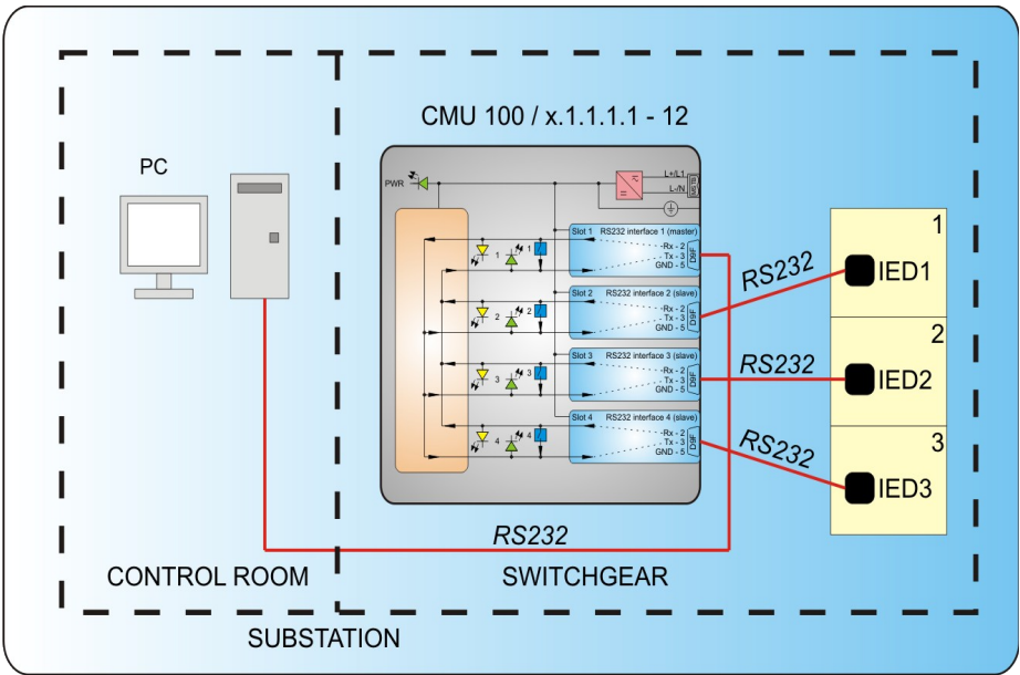
Picture 2: CMU 100 / x.1.1.1.1 - 12 typical application
