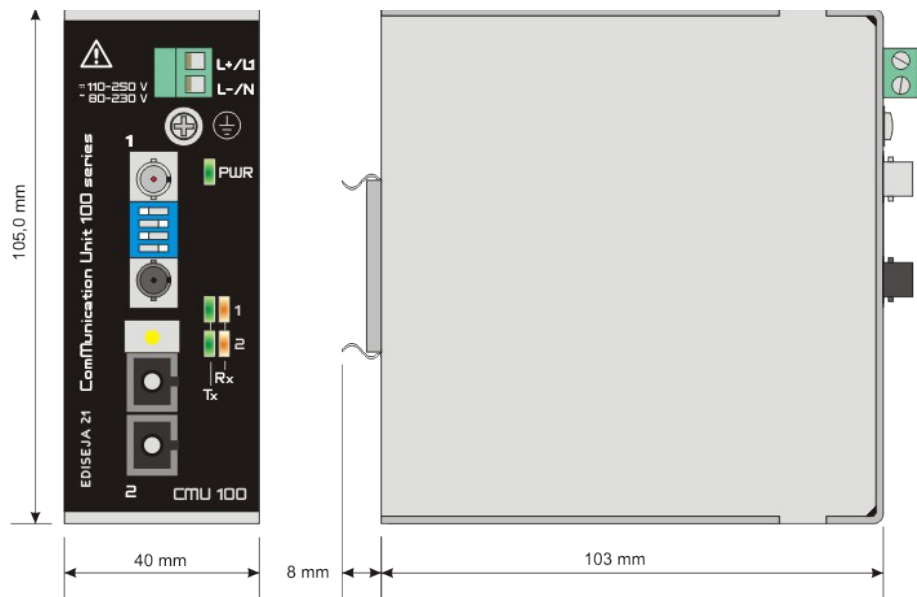
Picture 8: Dimensions
