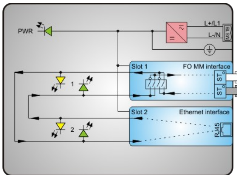
Picture 17: General diagram
