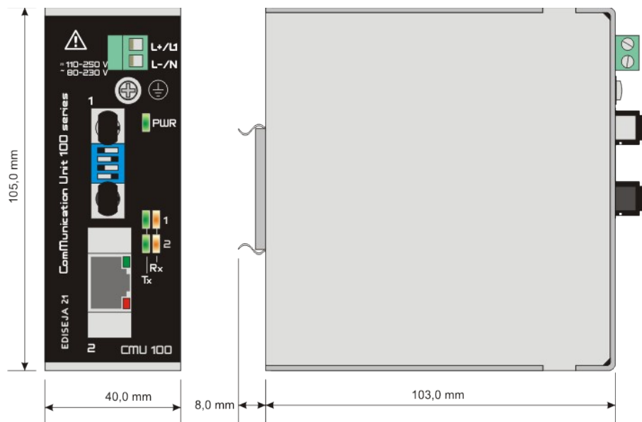
Picture 19: Dimensions
