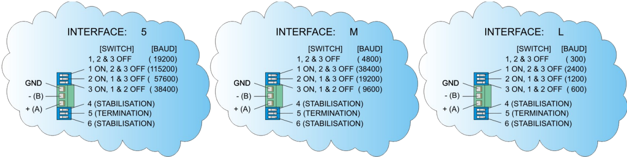
Picture 6: RS485 interface board appearance with switch settings
