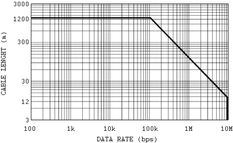
Picture 7: Standard data rate vs cable length
