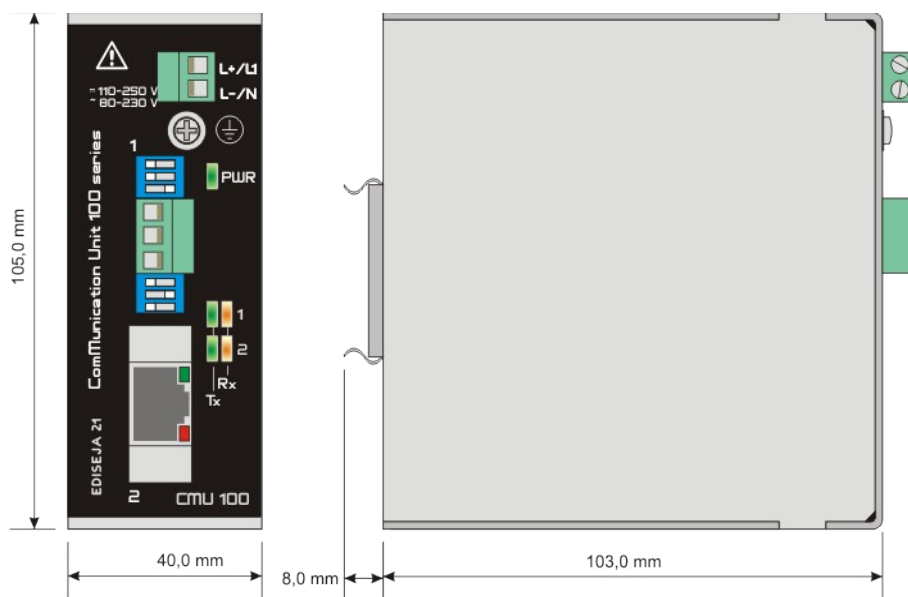
Picture 21: Dimensions
