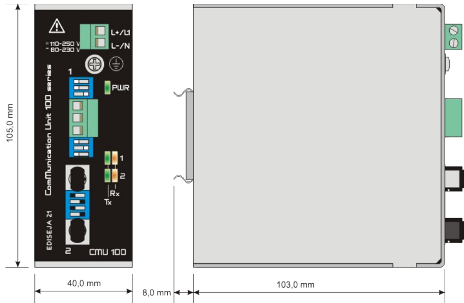
Picture 10: Dimensions
